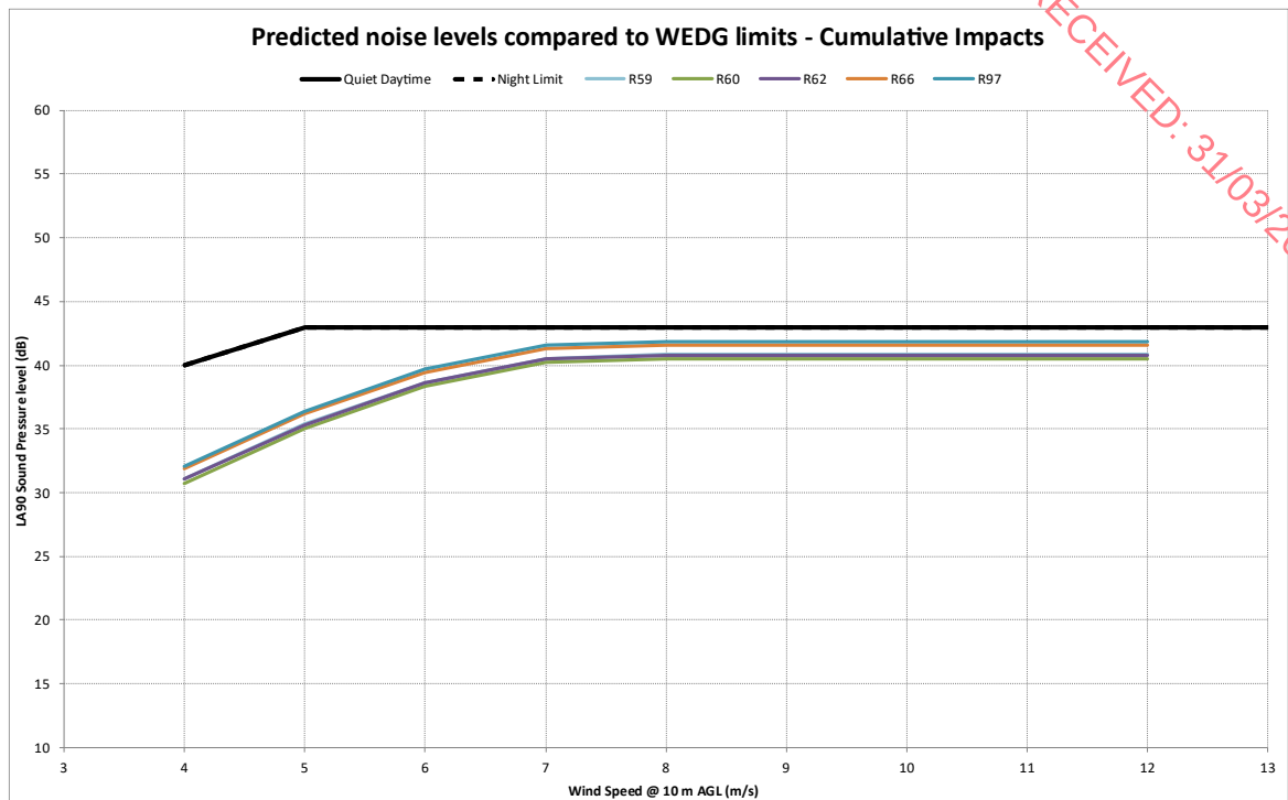
Figure 1-6: NML3 – Proposed Development Cumulative
